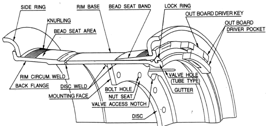
Diagram of a 5-Piece Earthmover Wheel fitted with a Flat Plate Centre Disc
