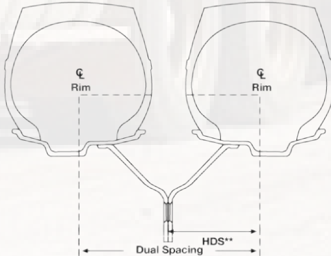
DUAL DISC WHEELS
