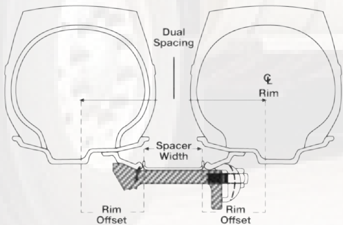
DUAL DEMOUNTABLE RIMS
