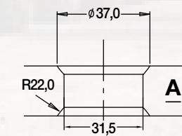
American/Japanese R22 Ball Taper for Double Cap Nut
