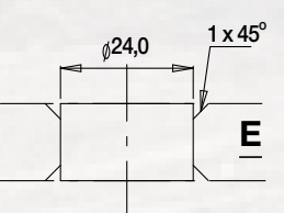
ISO No Countersink for Two-Piece Flange Nut
